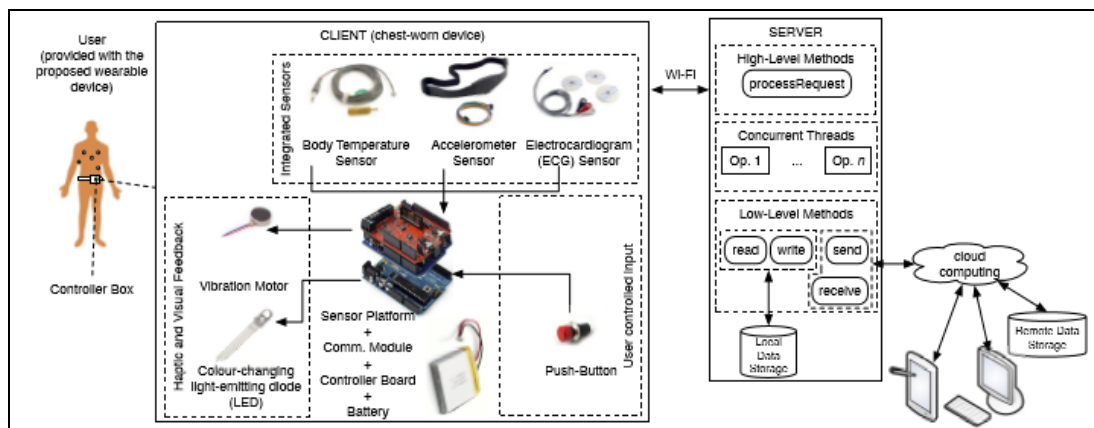
Fig 2: The proposed system architecture of the wearable multi-sensor fusion health-monitoring system.
