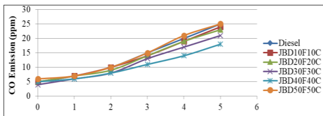
Fig 2: Load vs CO Emission
